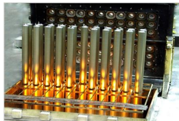
Wagstaff casting machine
